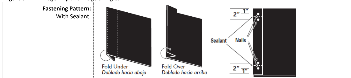
Figure 9 - RIZERidge® Hip and Ridge Shingles
