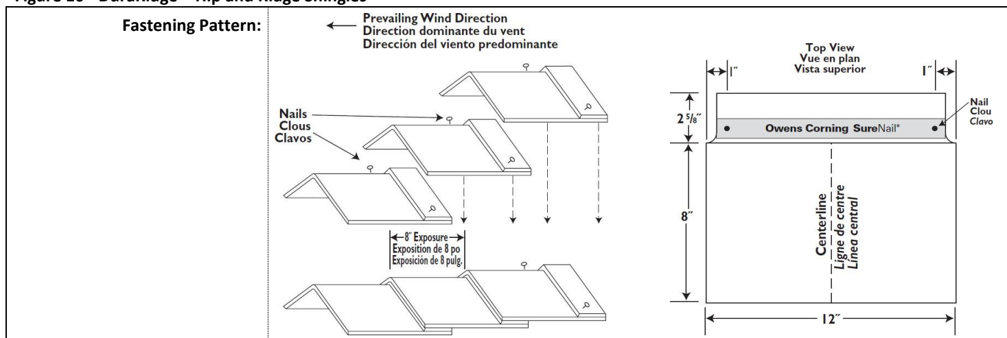
Figure 10 - DuraRidge™ Hip and Ridge Shingles
